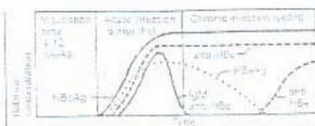
Fig. 12b Spontaneous fall of HBeAg in HBsAg carriers and the appearance of Anti HBe (with seroconversion).
